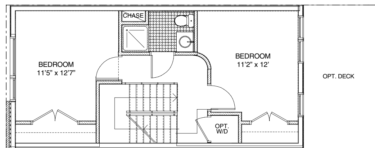
SECOND FLOOR
