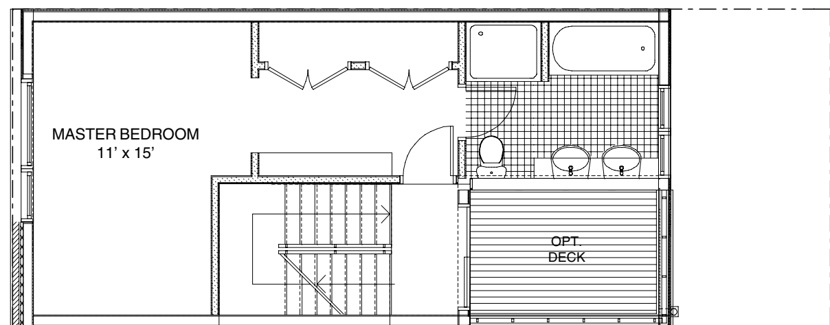
THIRD FLOOR
