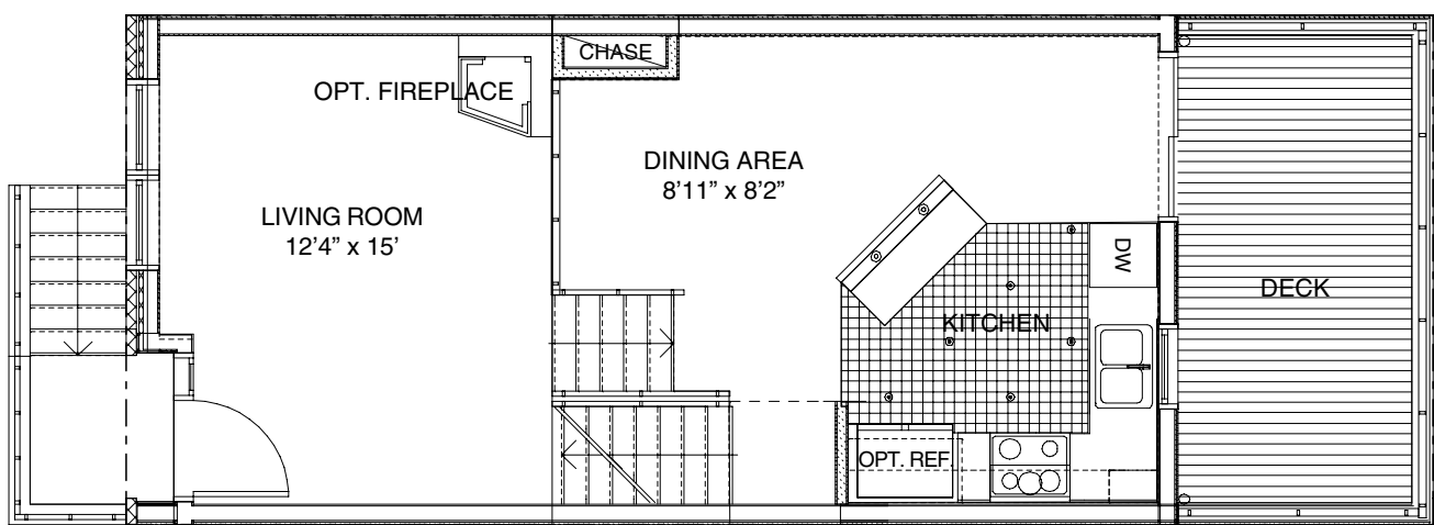
FIRST FLOOR
