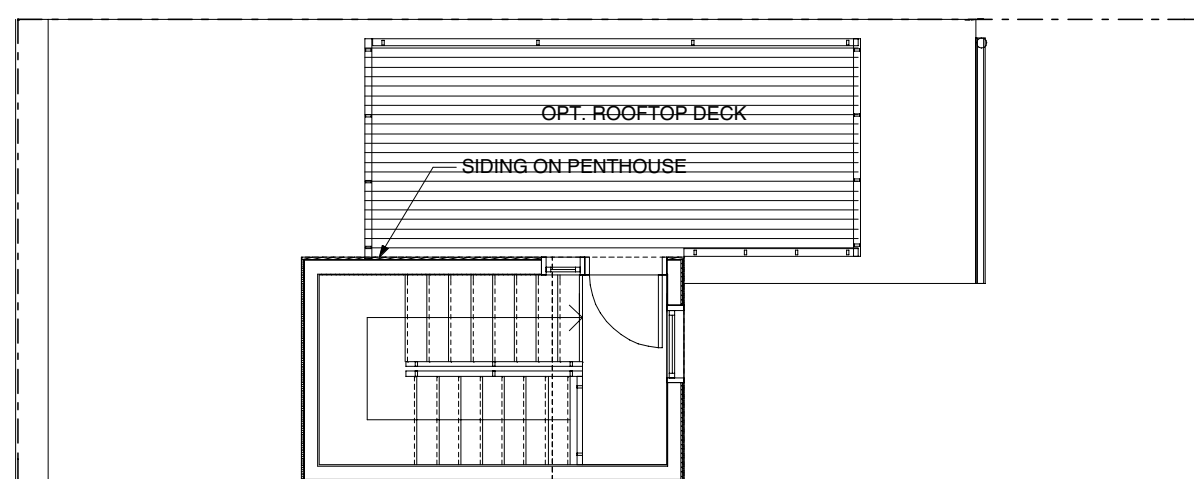
ROOF PLAN
